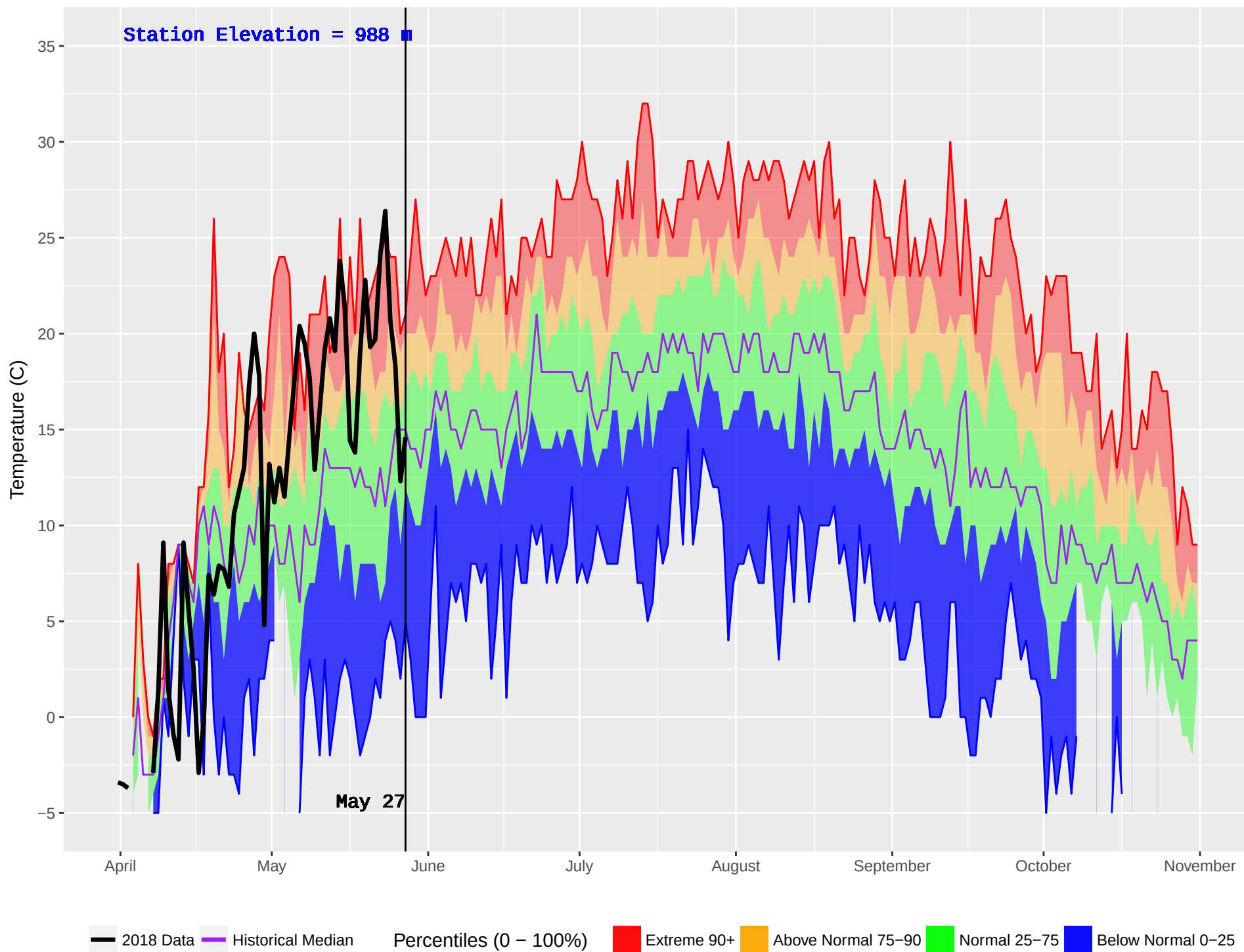
NOEL (437) : Historical (1993–2016) and Current (2018) Noon Temperature
