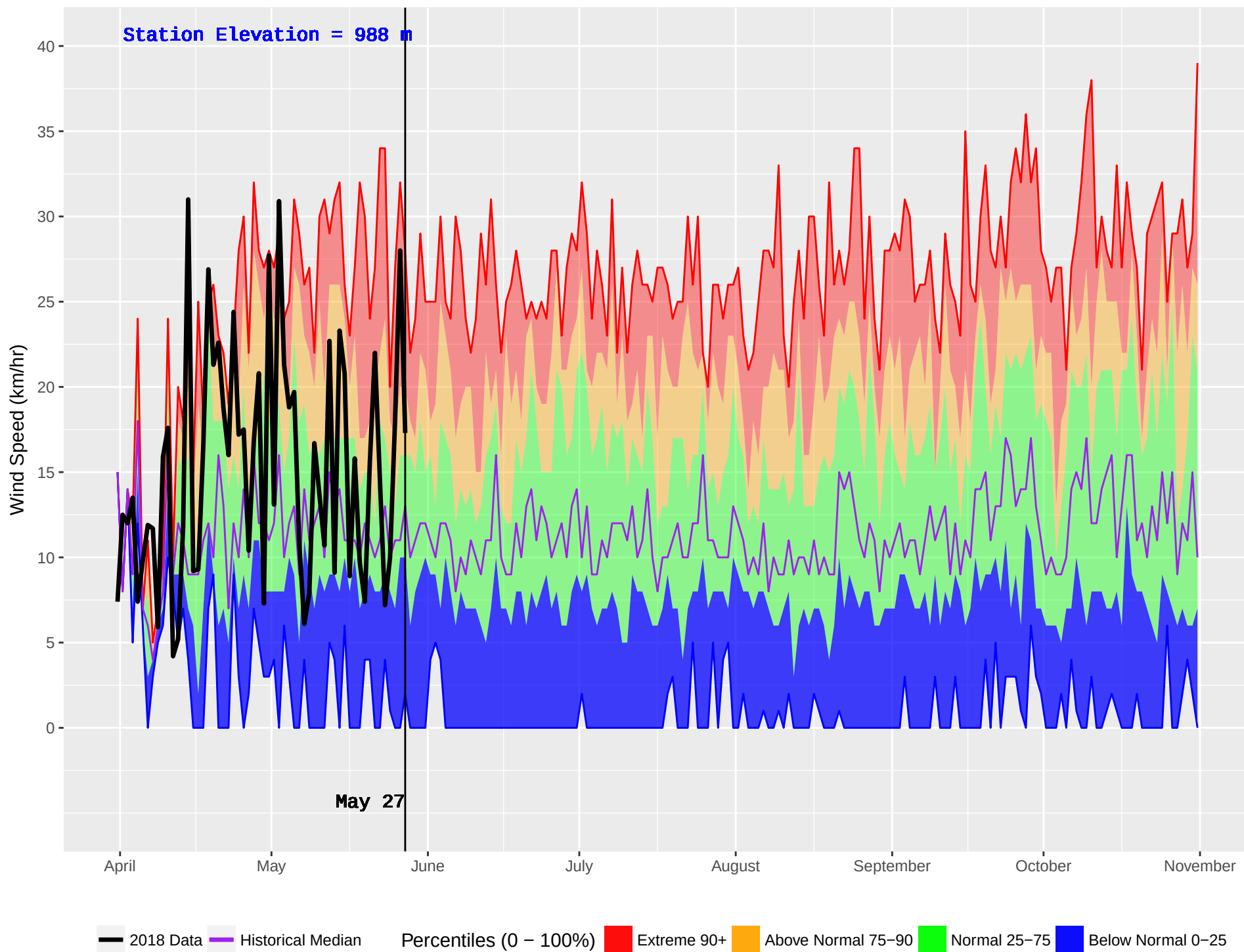
NOEL (437) : Historical (1993–2016) and Current (2018) Noon Wind Speed
