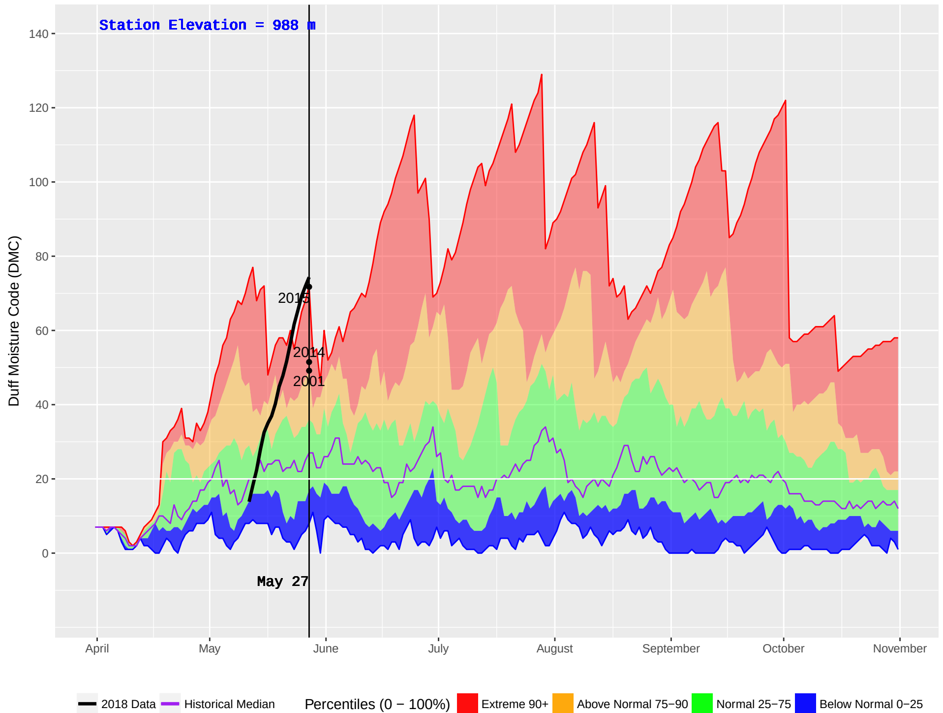
NOEL (437) : Historical (1993–2016) and Current (2018) Noon Duff Moisture Code (DMC)
