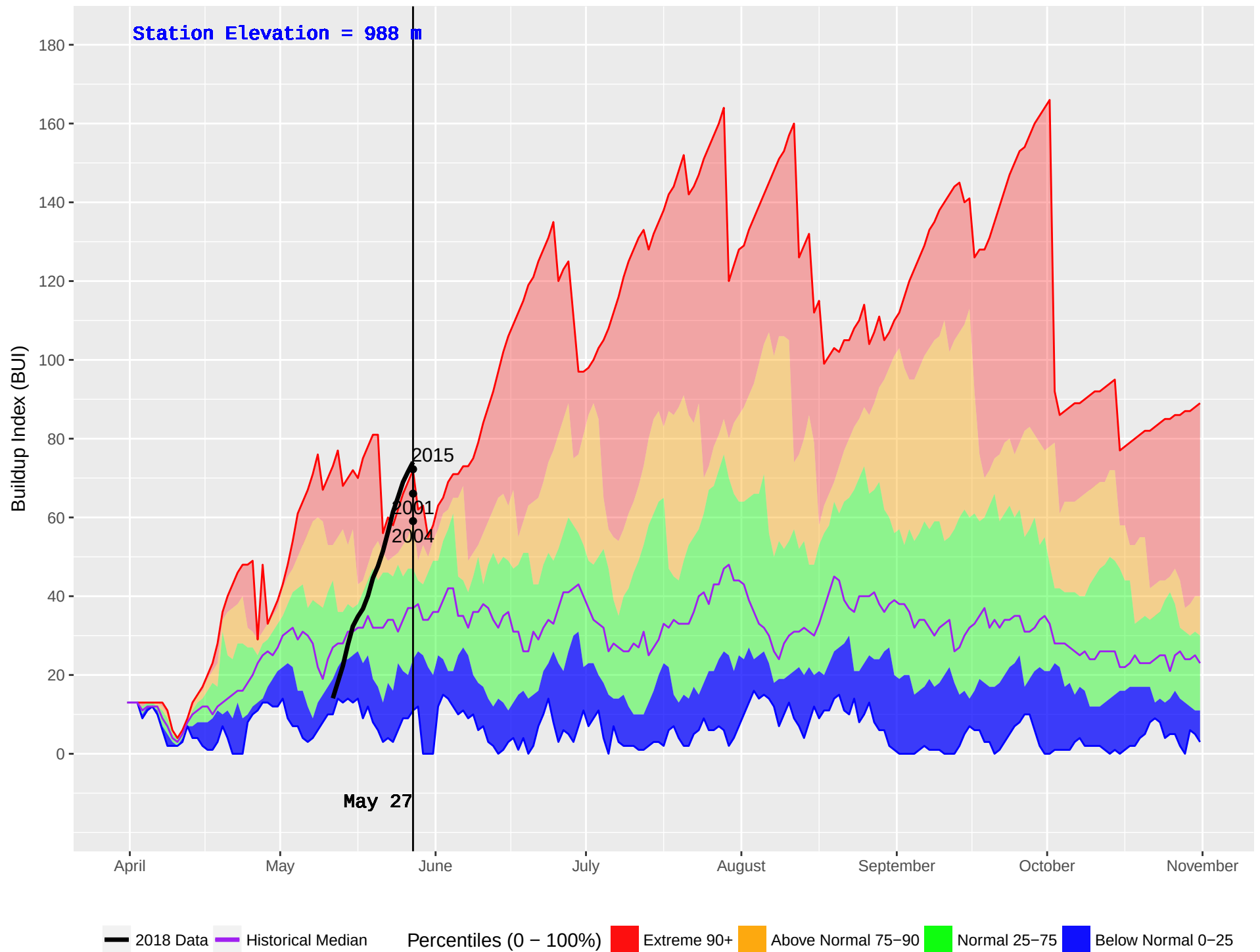
NOEL (437) : Historical (1993–2016) and Current (2018) Noon Buildup Index (BUI)
