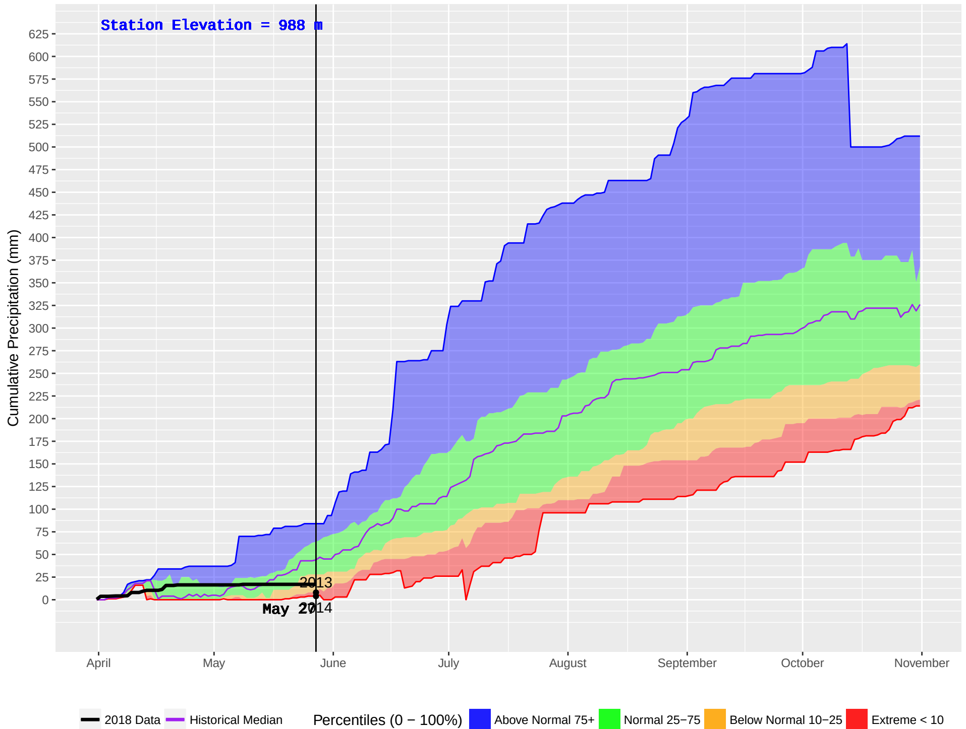
NOEL (437) : Historical (1993–2016) and Current (2018) Noon Cumulative Precipitation
