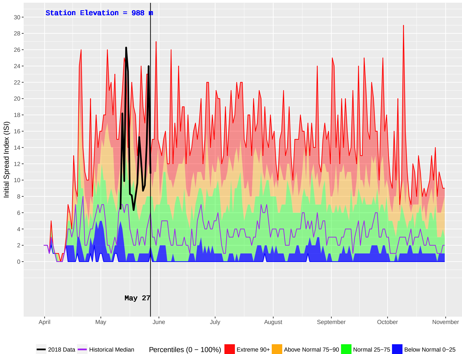
NOEL (437) : Historical (1993–2016) and Current (2018) Noon Initial Spread Index (ISI)
