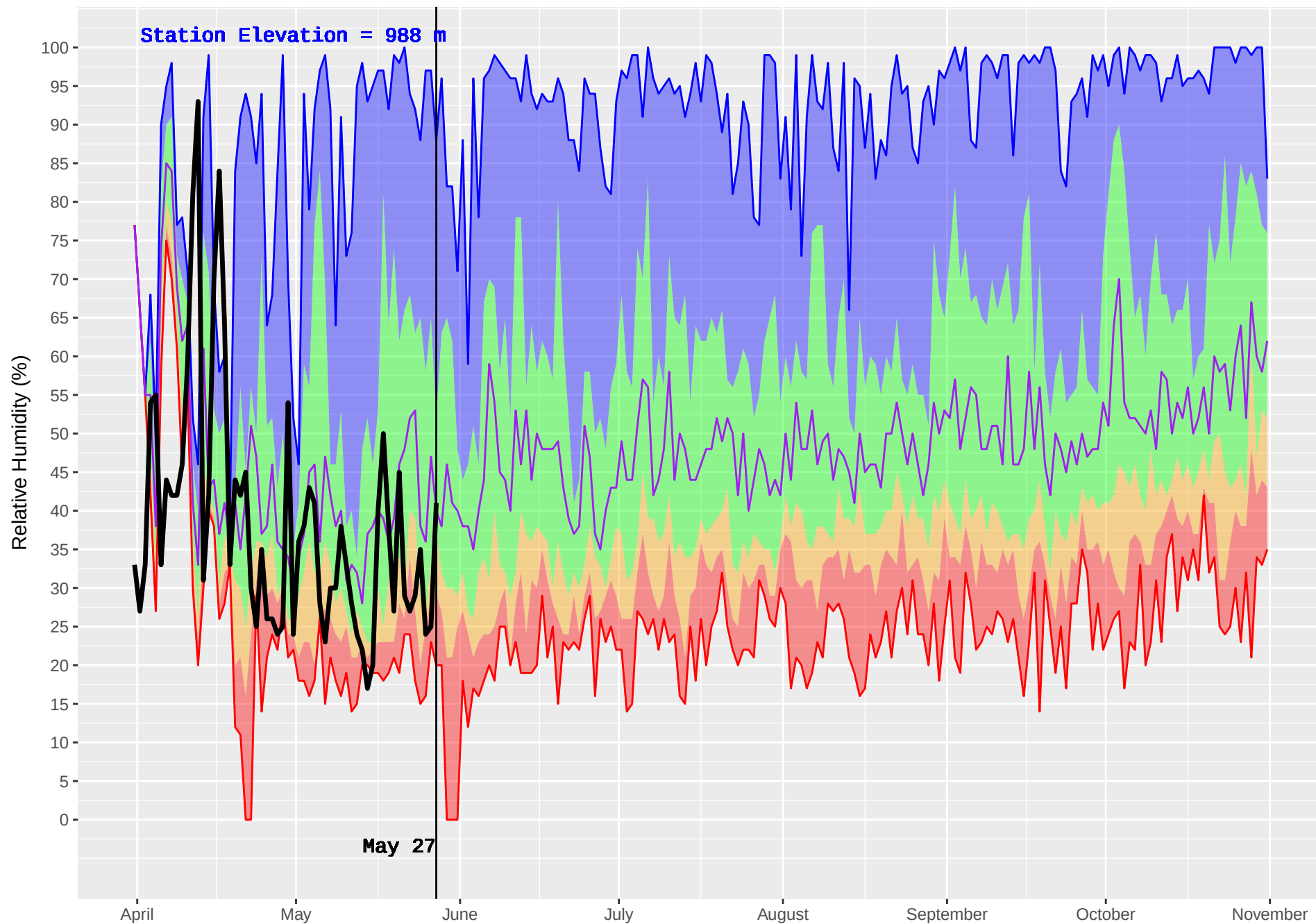
NOEL (437) : Historical (1993–2016) and Current (2018) Noon Relative Humidity
