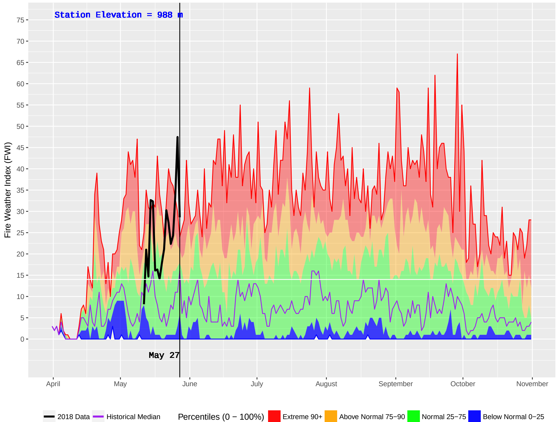
NOEL (437) : Historical (1993–2016) and Current (2018) Noon Fire Weather Index (FWI)
