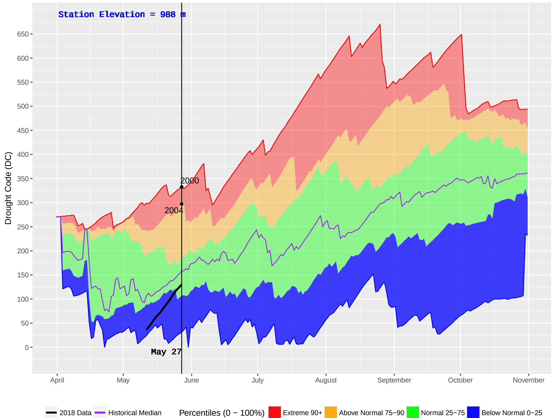
NOEL (437) : Historical (1993–2016) and Current (2018) Noon Drought Code (DC)
